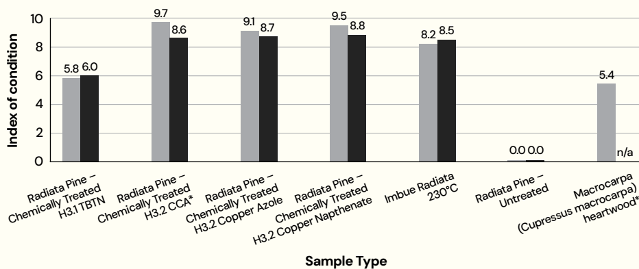
Graph 1: Decking Panels – Condition After 11 Years
