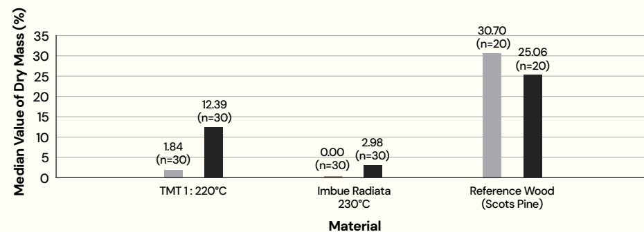
Graph 5: Mass Losses and Corresponding Durability Classes of Heat Tempered Radiata Pine
